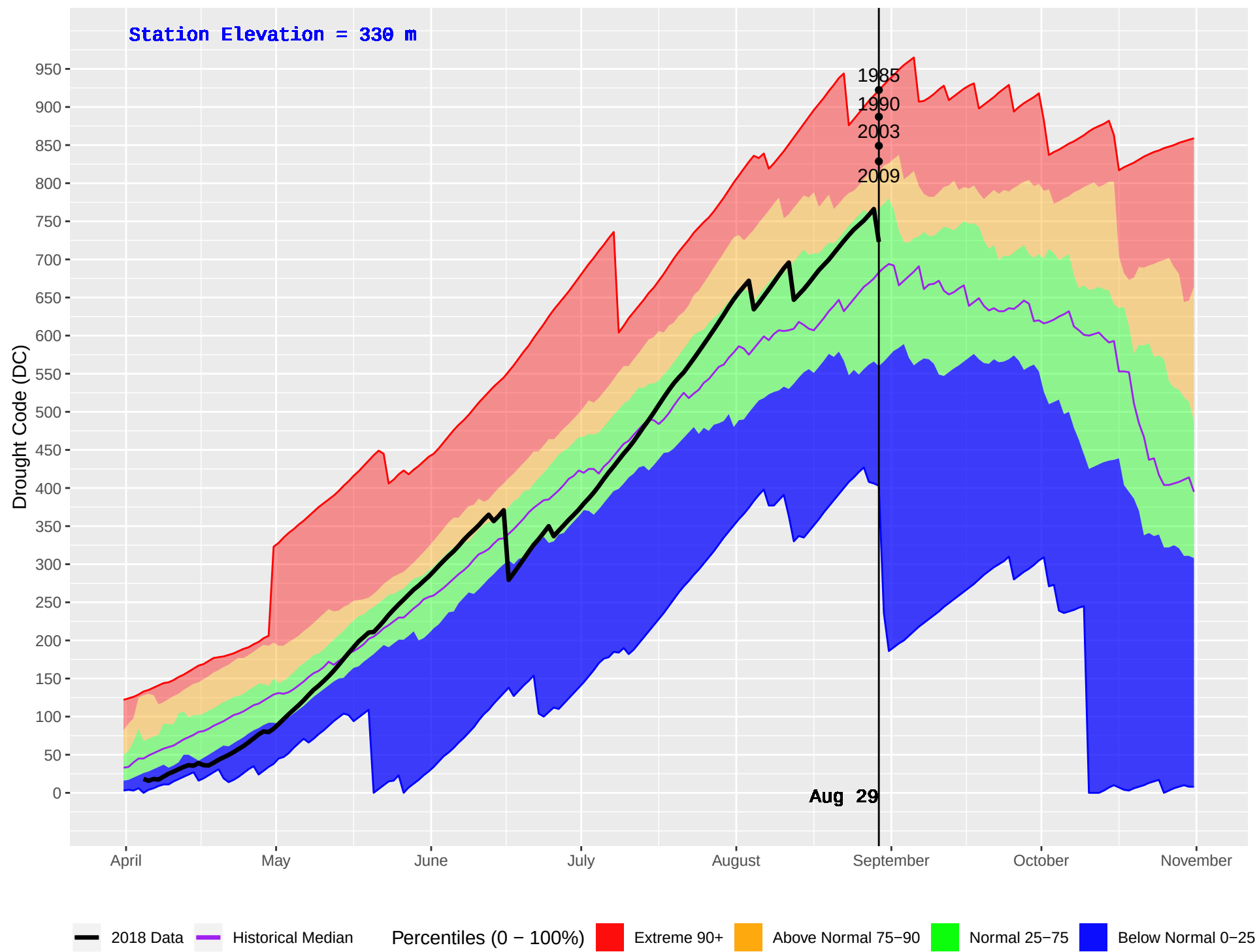
D'ARCY (292) : Historical (1978–2016) and Current (2018) Daily Drought Code (DC)
