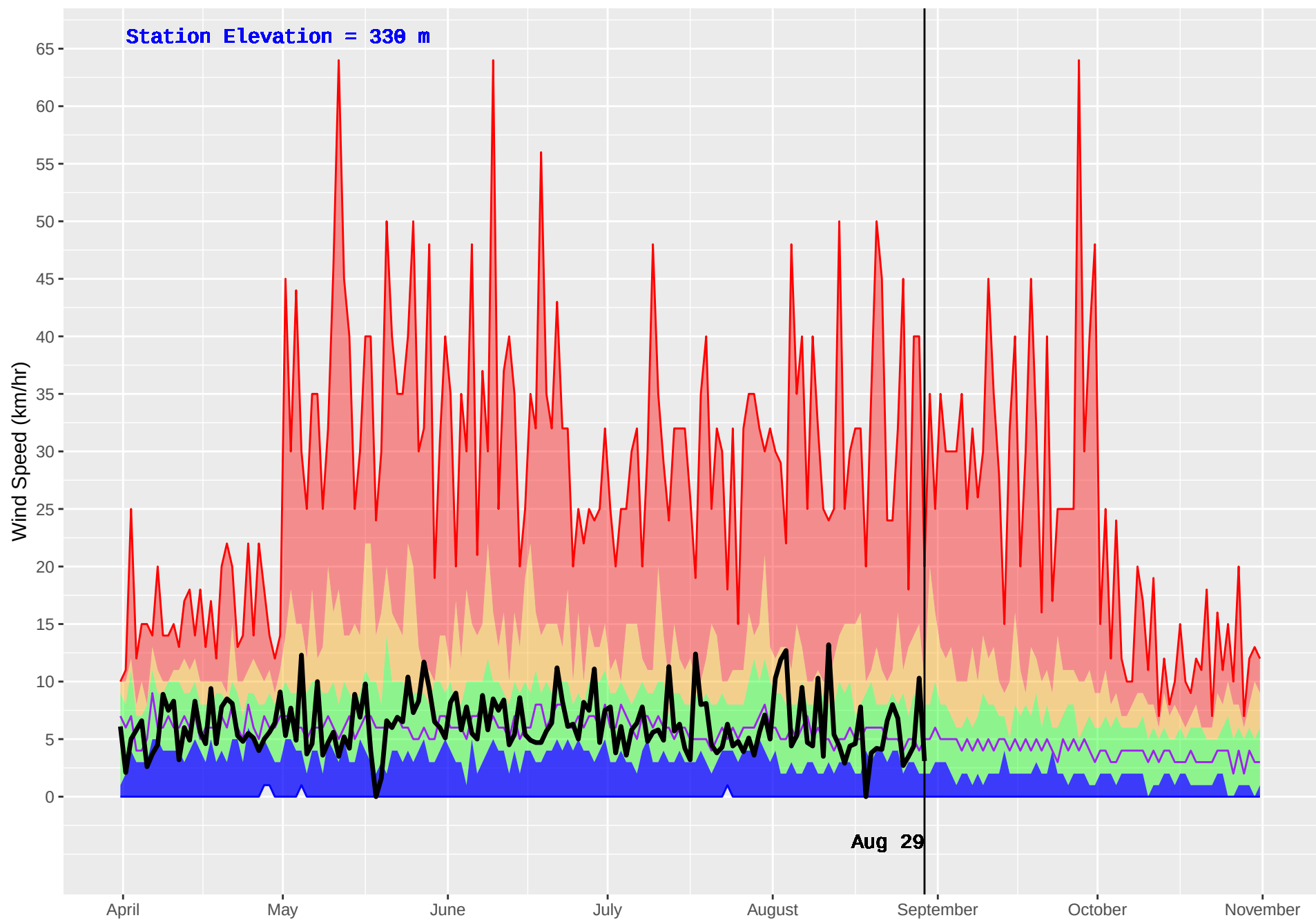
D'ARCY (292) : Historical (1978–2016) and Current (2018) Daily Wind Speed
